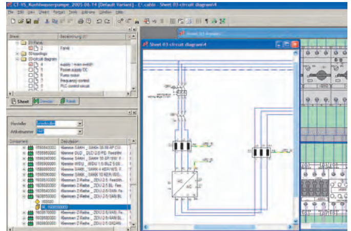
Example of a circuit diagram
