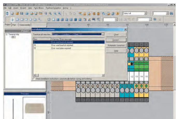
Plausibility check of the terminal rail design in RailDesigner®
