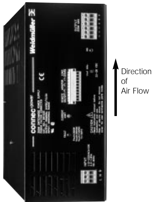
Figure 2 Vertical Mount
